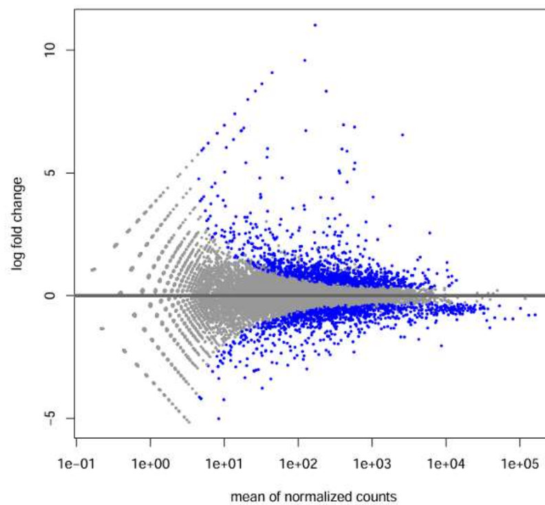
MA-plot for condition: 5thXdayXinfected vs FactorLevel
