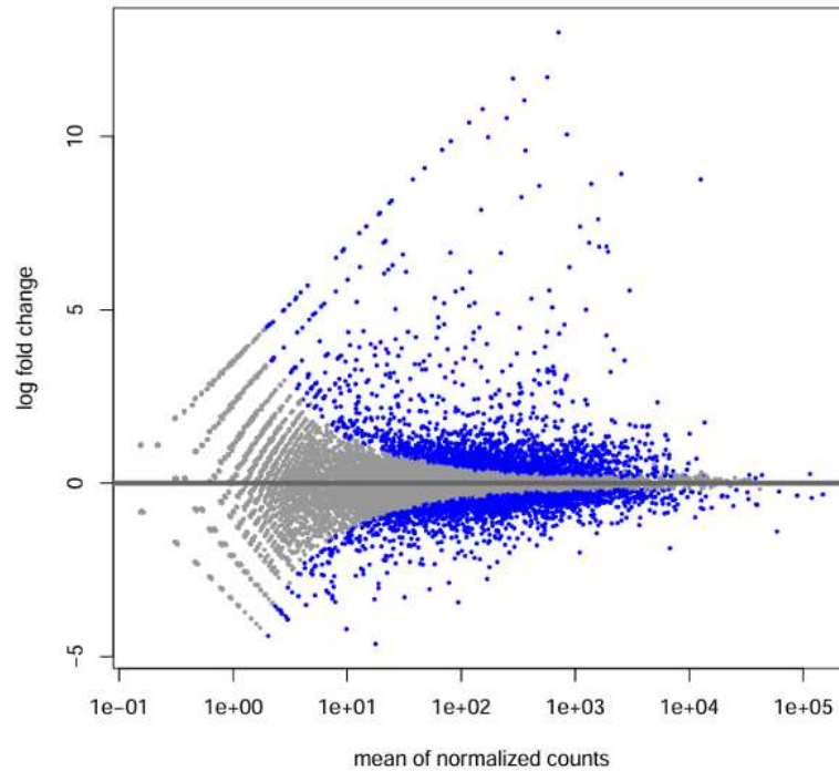
MA-plot for condition: 3rdXdayXinfected vs Control
